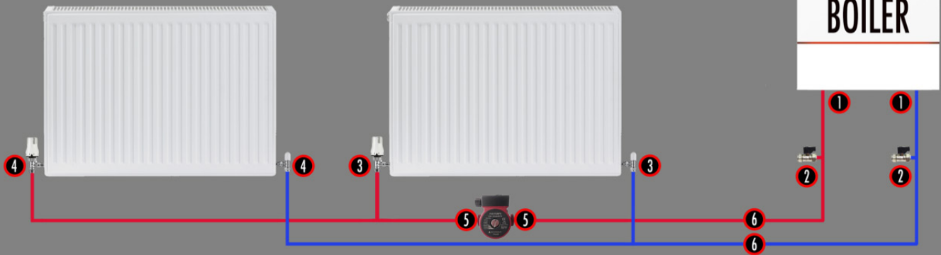
Fig 1: Connecting the Thoroughflush to the Heating System
