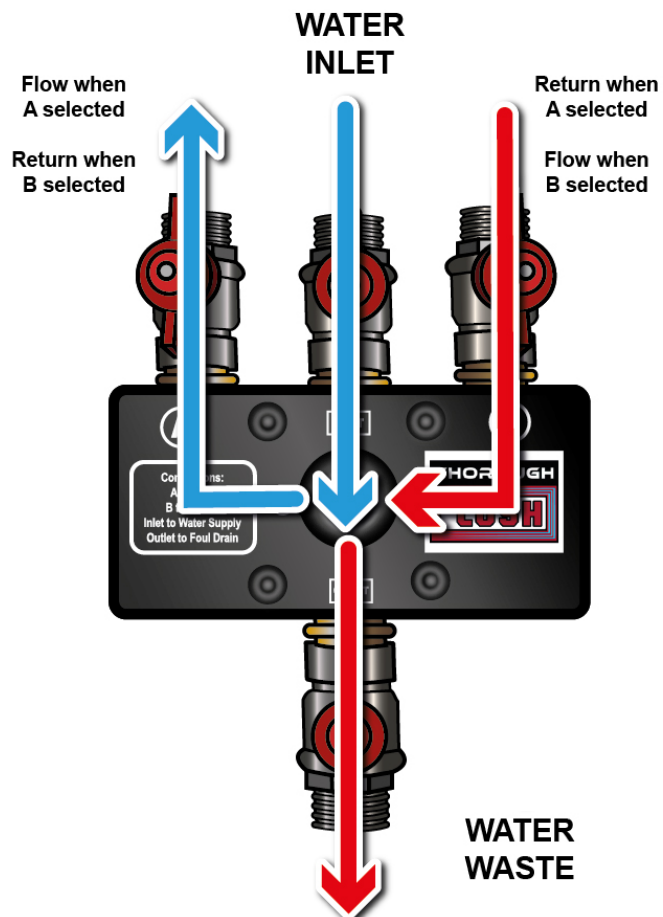
Fig 2: Thoroughflush connections
